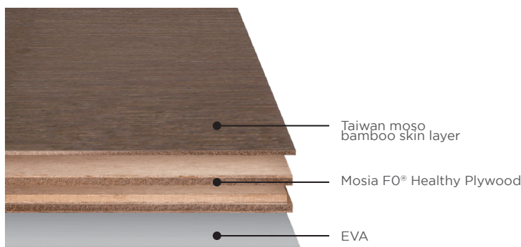
Composite Bamboo Flooring Structure
